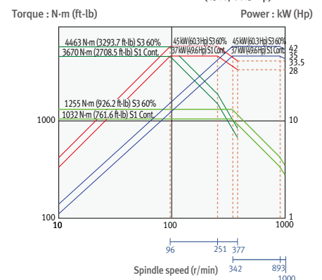
PUMA 480D [LD/XLD] (37/45 KW) (49.6/60.3 Hp)
